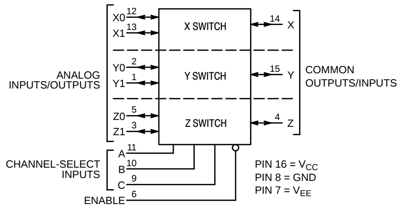
Triple Single-Pole, Double-Position Plus Common Off
