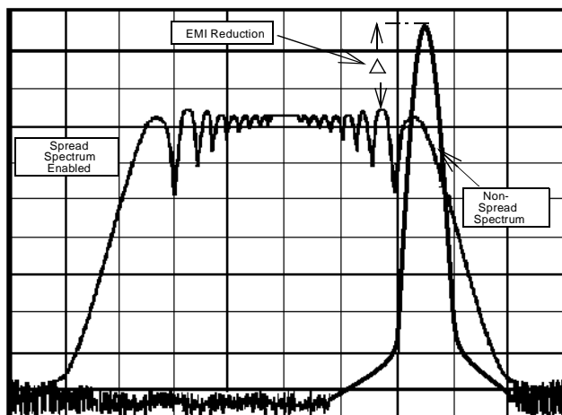
Figure 5. Typical Clock and SSFTG Comparison
