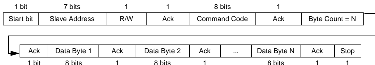
Figure 7. An Example of a Block Write [6]
