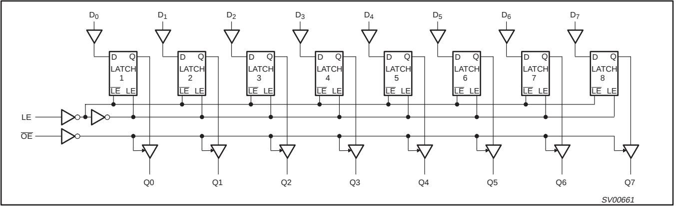
LOGIC DIAGRAM
