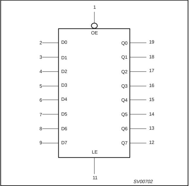
LOGIC SYMBOL
