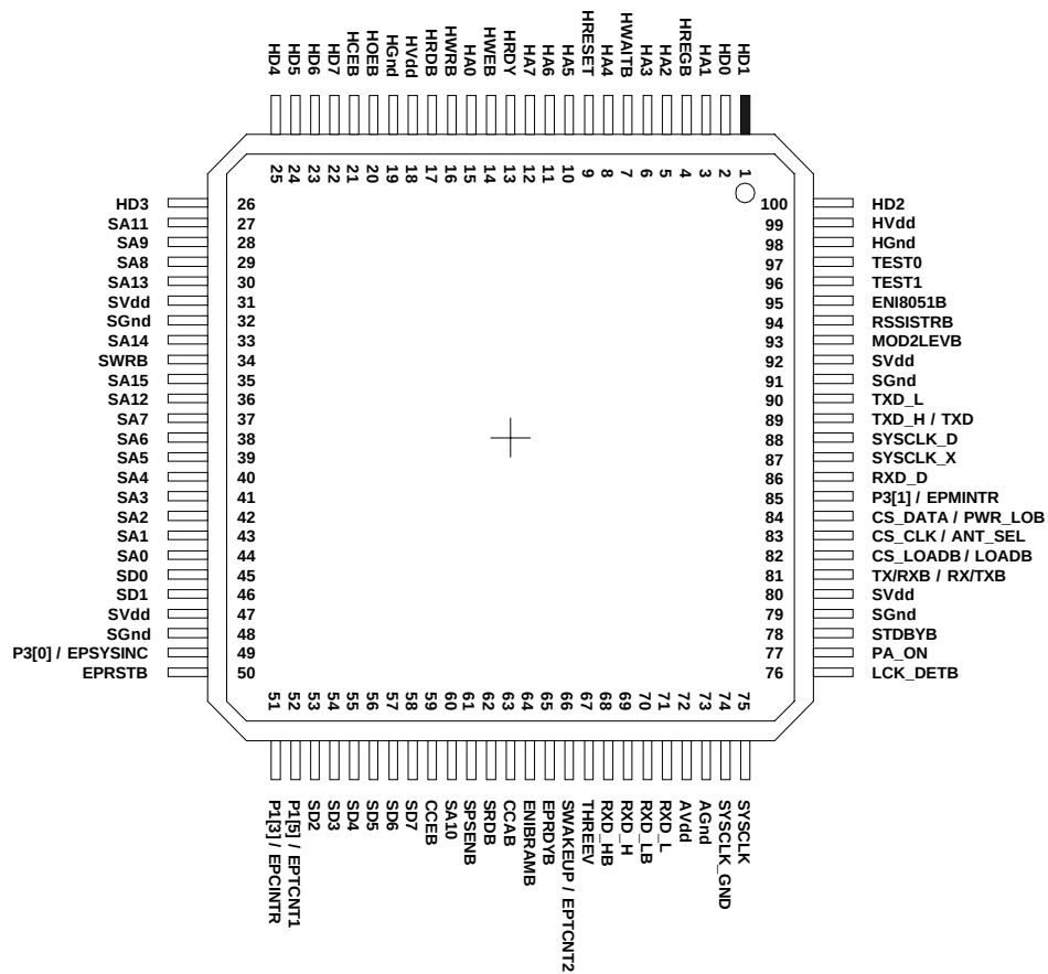
Fig.ure 2 100 Pin package
