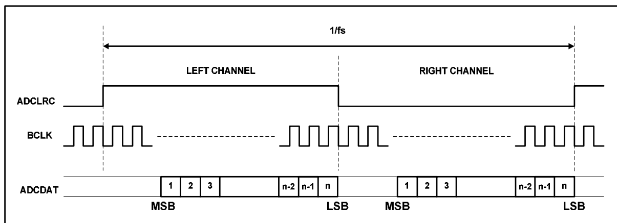
Figure 19 Right Justified Mode
