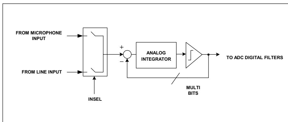
Figure 14 Multi-Bit Oversampling Sigma Delta ADC Schematic
