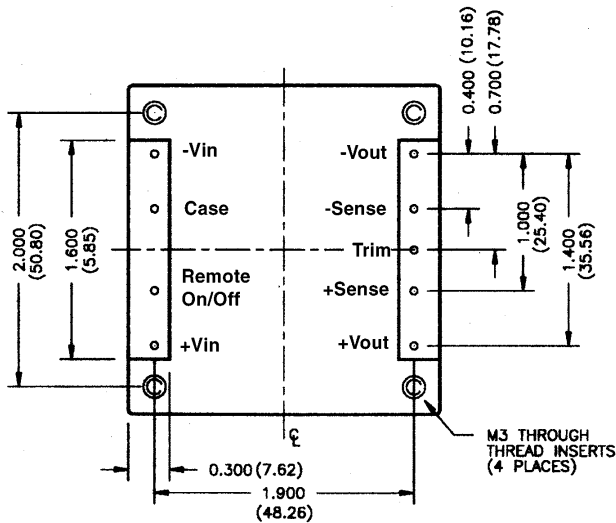
SINGLE BOTTOM VIEW
