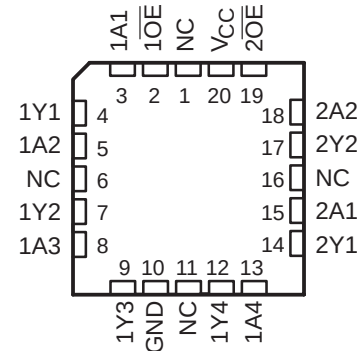
SN54HC367 . . . FK PACKAGE (TOP VIEW)
