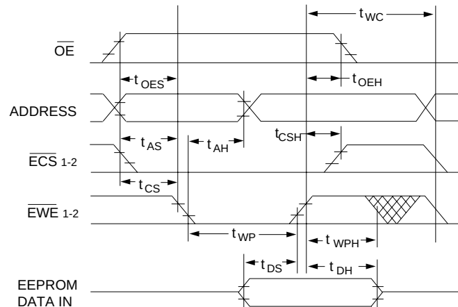
FIG. 8 EEPROM WRITE WAVEFORMS ECS CONTROLLED
