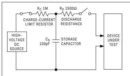
Figure 2a. Human Body ESD Test Model
