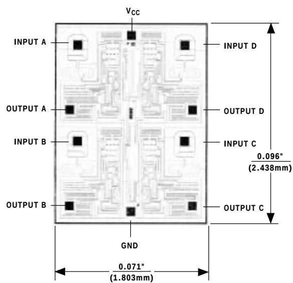
Chip Topography
