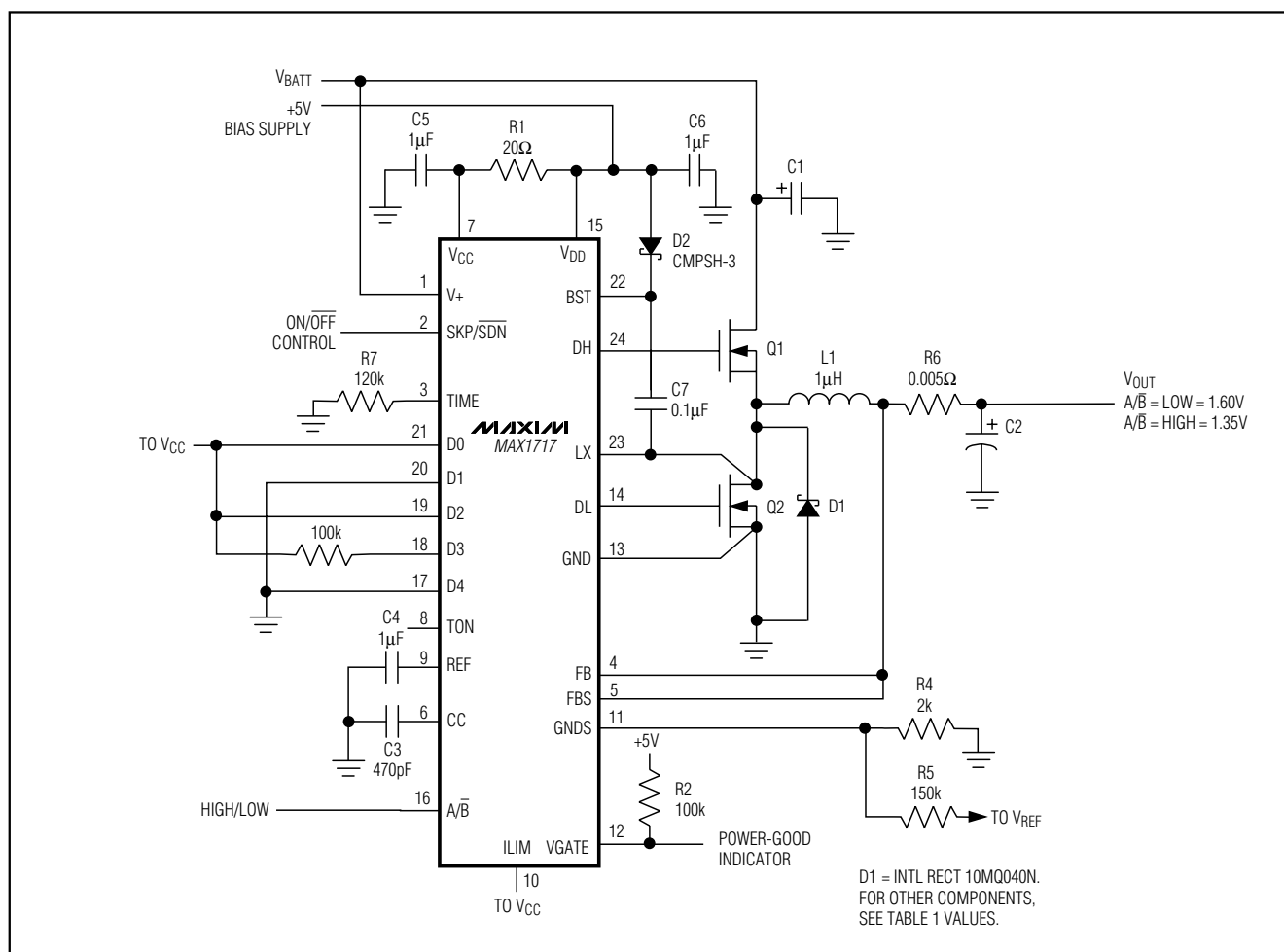
Figure 3. Voltage-Positioned Circuit
