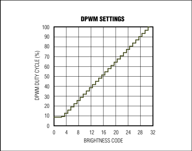
Figure 5. DPWM Settings
