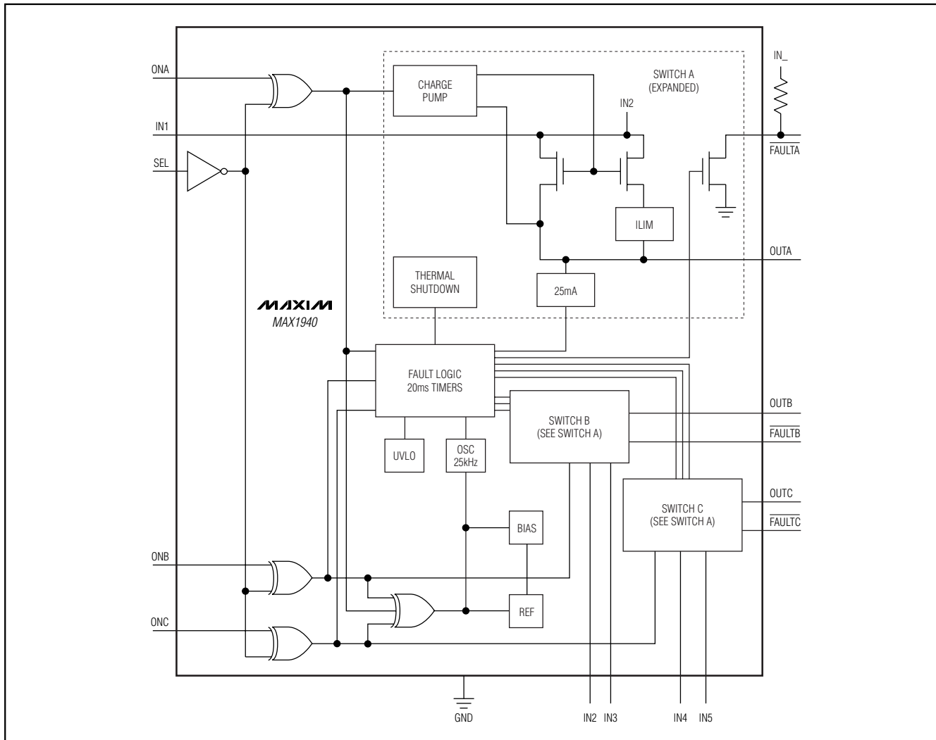
Figure 1. Functional Diagram
