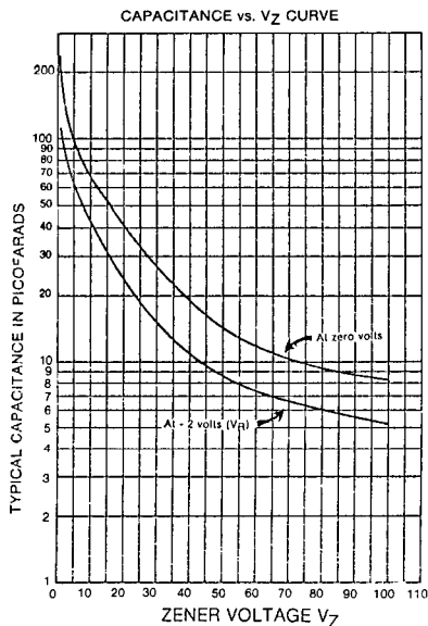
FIGURE 4 CAPACITANCE VS. ZENER VOLTAGE (TYPICAL)
