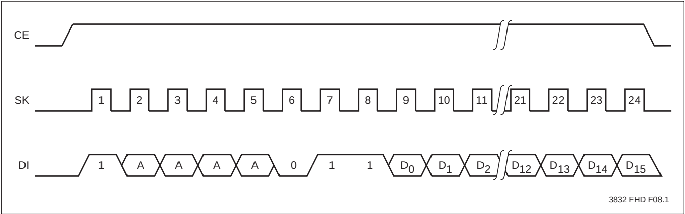
Figure 2. RAM Write
