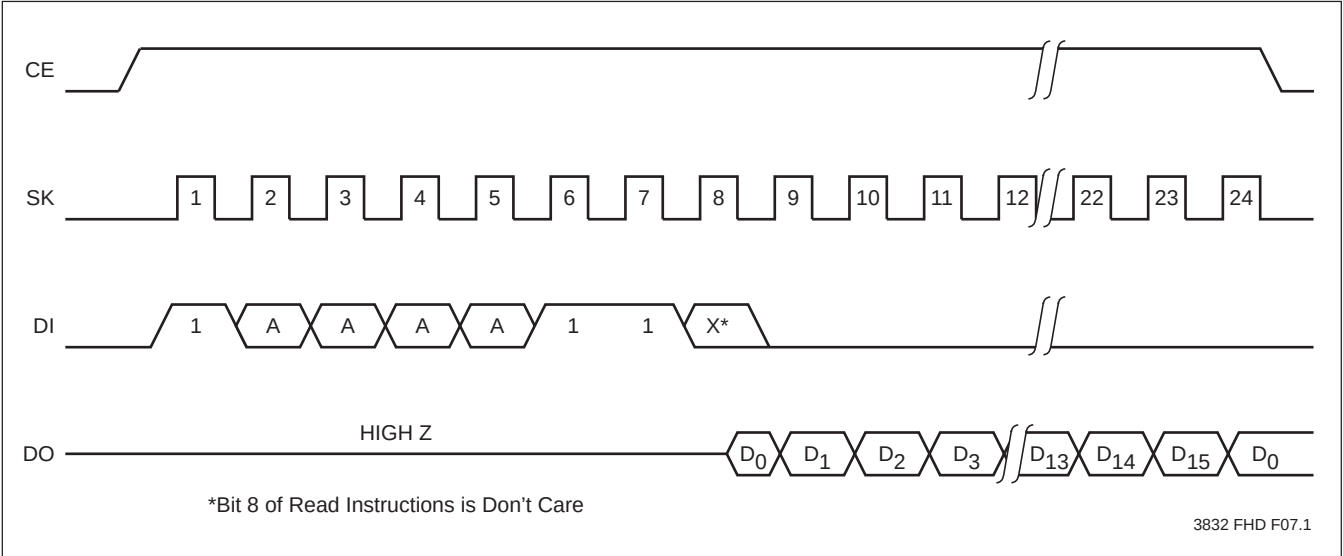
Figure 1. RAM Read
