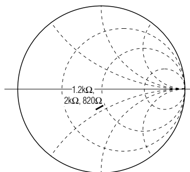
MAX2683 LOX2 S11 vs. R_{BIAS} ( \overline{ENX2} = GND )
