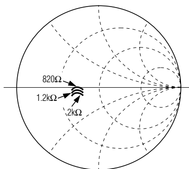
LOX1 S11 vs. R_{BIAS} ( \overline{ENX2} = V_{CC} )
