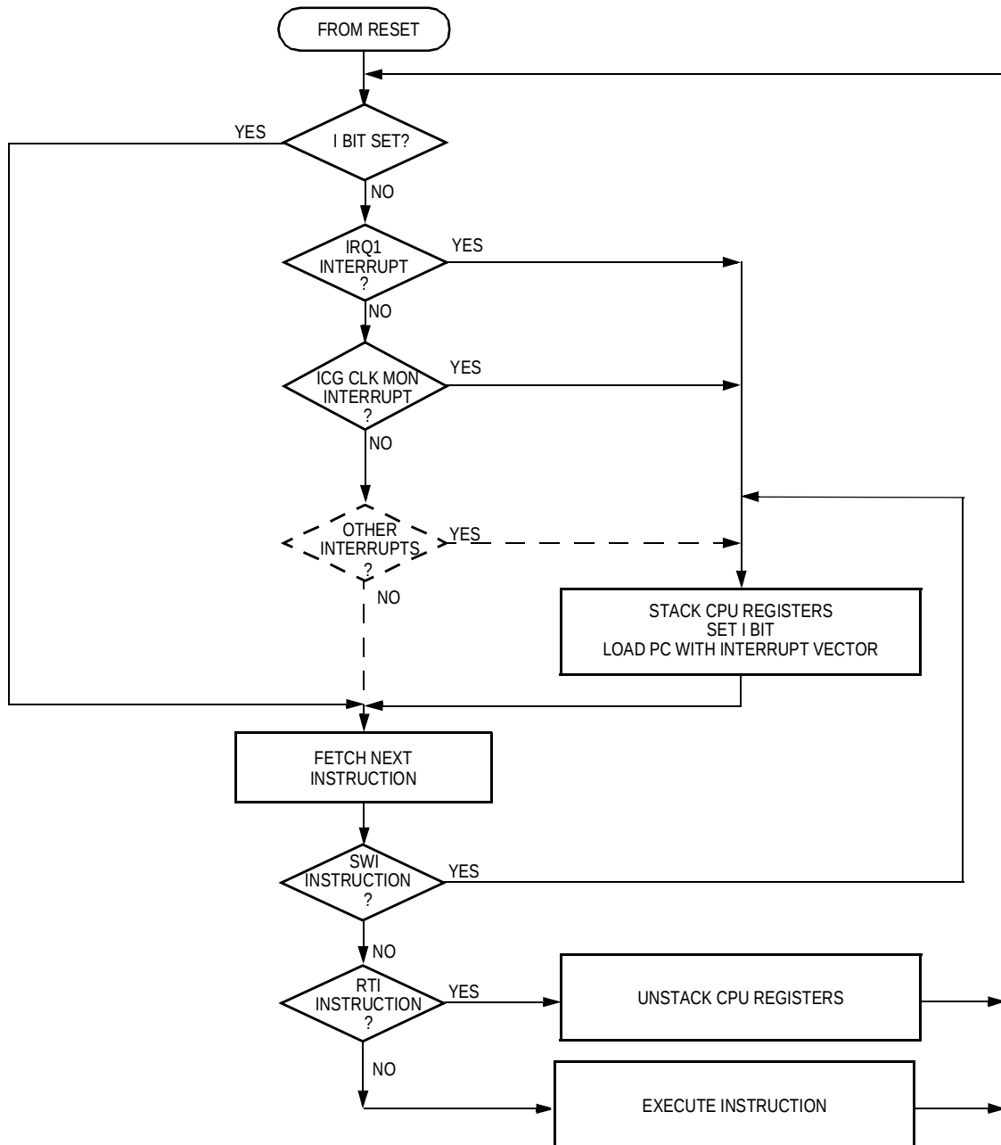
Figure 6-9. Interrupt Processing
