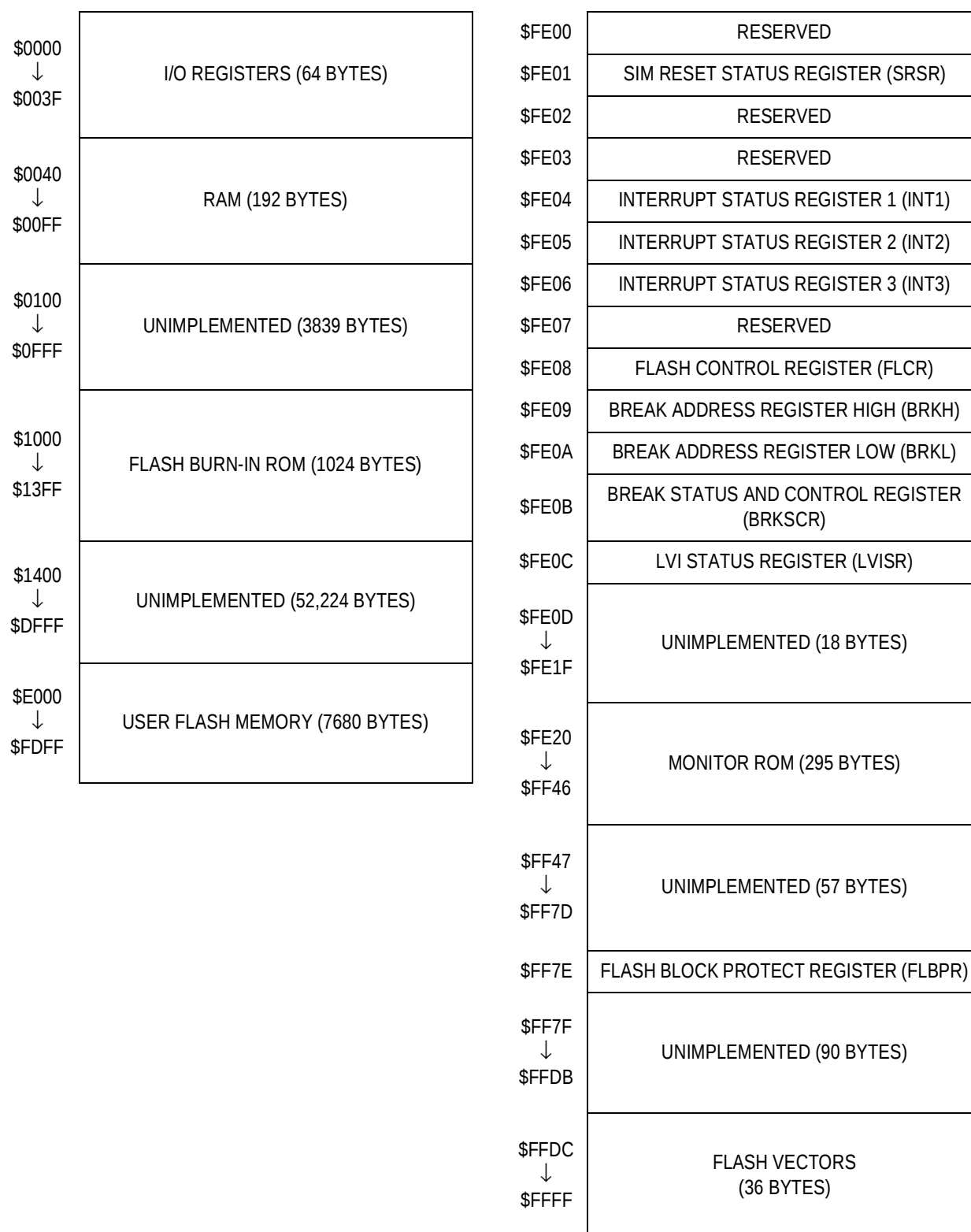
Figure 2-1. Memory Map
