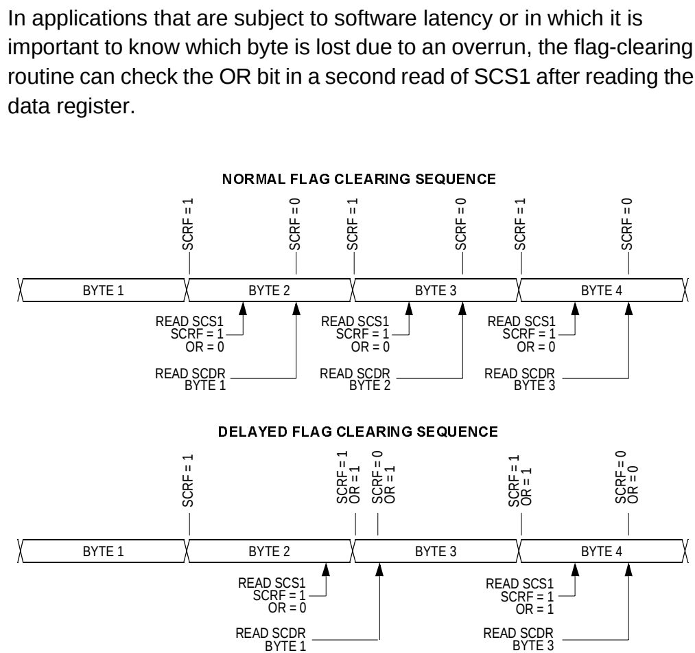
Figure 14-13. Flag Clearing Sequence
