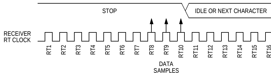
Figure 14-8. Fast Data
