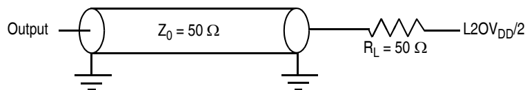
Figure 10. AC Test Load for the L2 Interface
