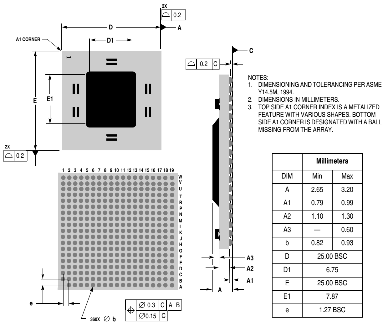
Figure 19. Mechanical Dimensions and Bottom Surface Nomenclature for the MPC755, 360 CBGA Package
