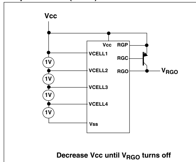
Sleep test circuit (X3100)
