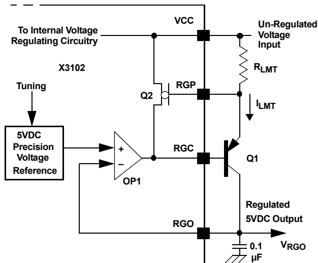
FIGURE 16. VOLTAGE REGULATOR OPERATION
