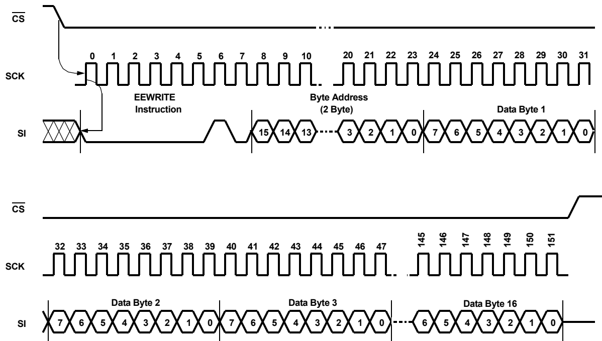
FIGURE 19. EEPROM PAGE WRITE (EWRITE) OPERATION SEQUENCE
