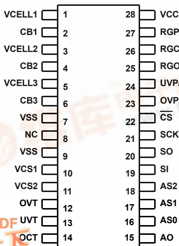
X3102 (TSSOP) TOP VIEW
