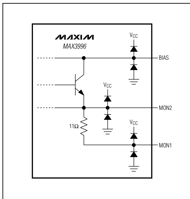
Figure 17. BIAS Output
