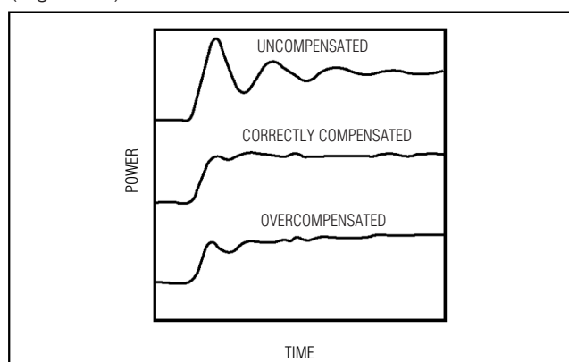
Figure 12. Laser Compensation
