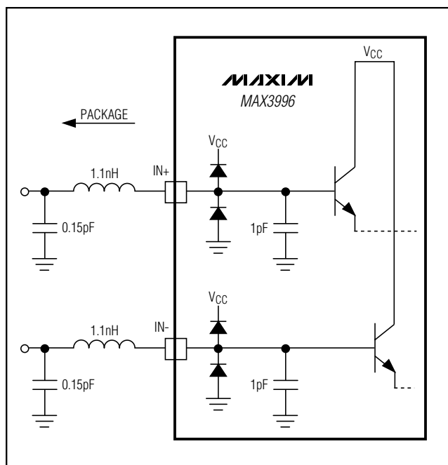
Figure 16. Data Inputs
