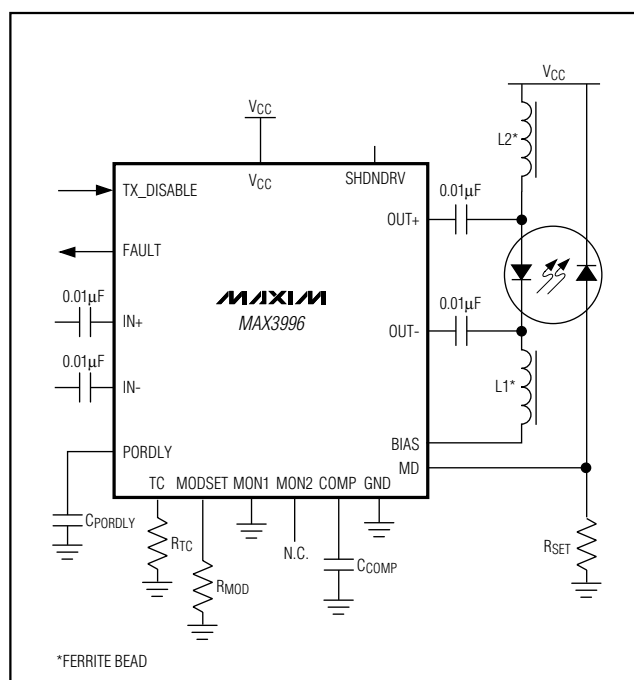
Figure 10. Differential Configuration
