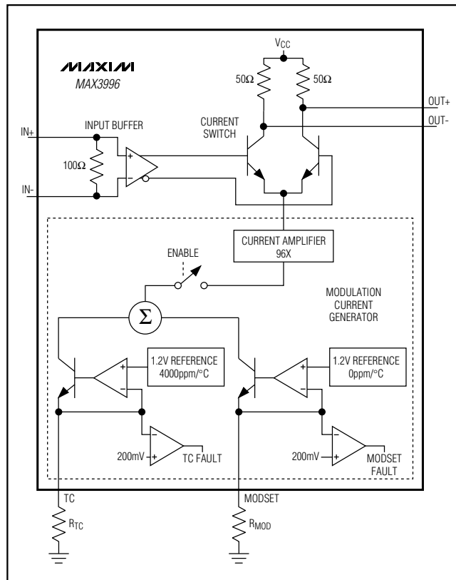
Figure 5. Modulation Circuitry
