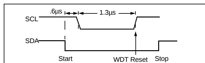
Figure 4. Watchdog Restart
