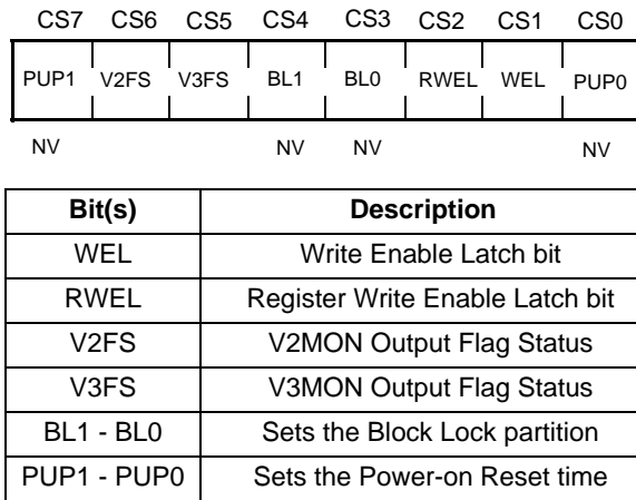
Figure 17. CR Register Format
