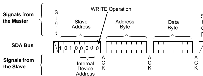
Figure 11. EEPROM Byte Write Sequence
