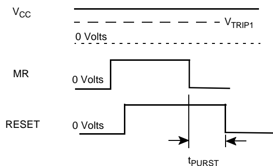
Figure 19. Manual Reset Response
