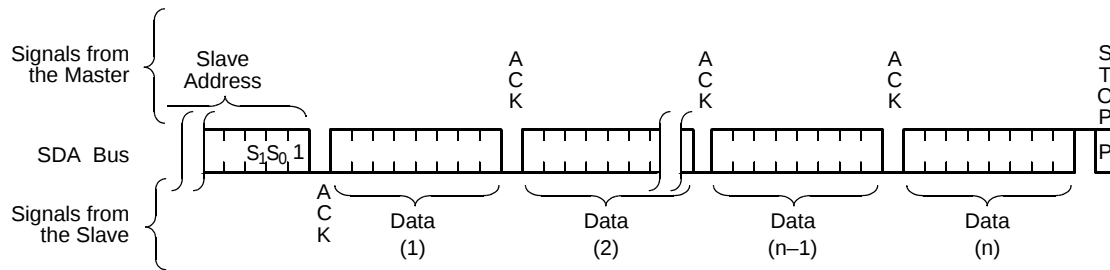
Figure 16. Sequential Read Sequence
