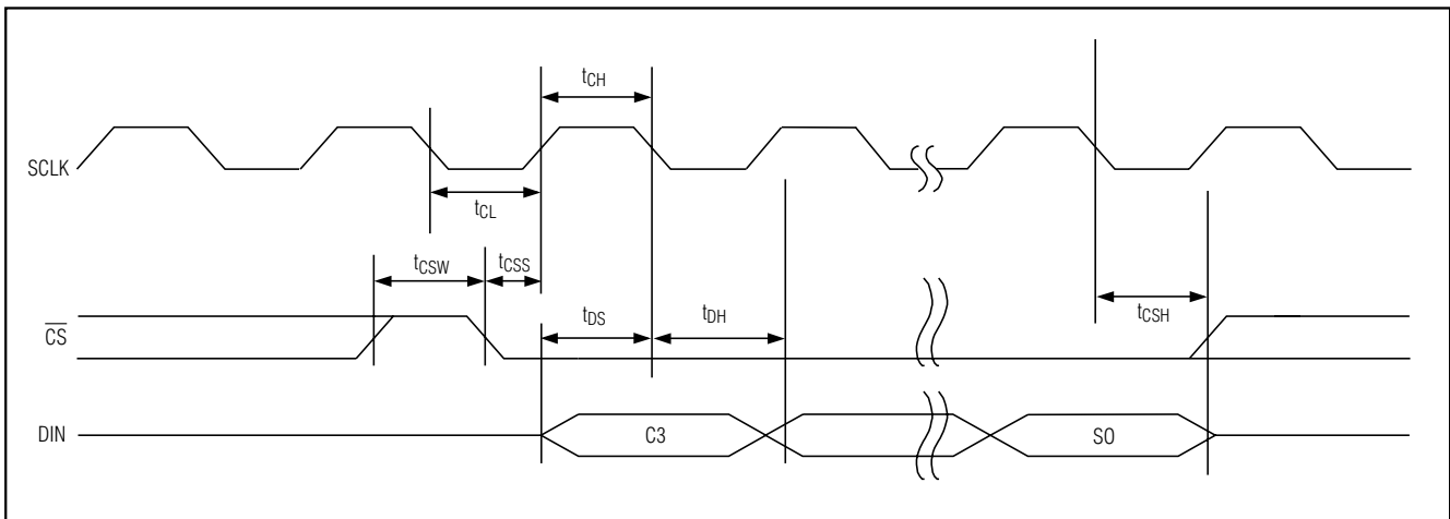
Figure 2. Timing Diagram
