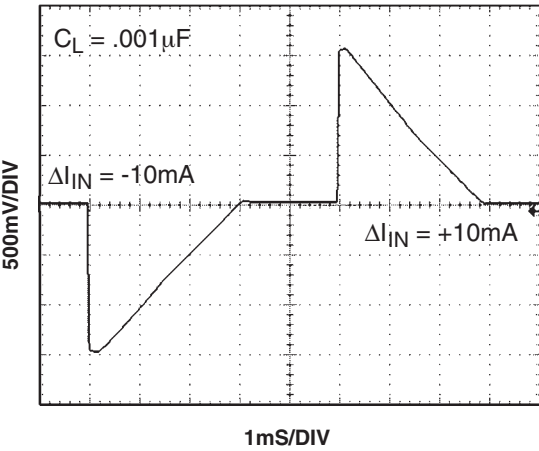
10mA LOAD TRANSIENT RESPONSE
