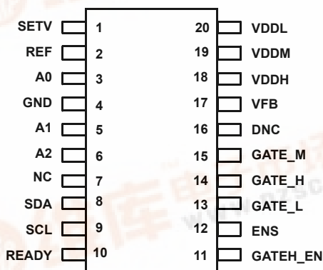
20 LD TSSOP TOP VIEW
