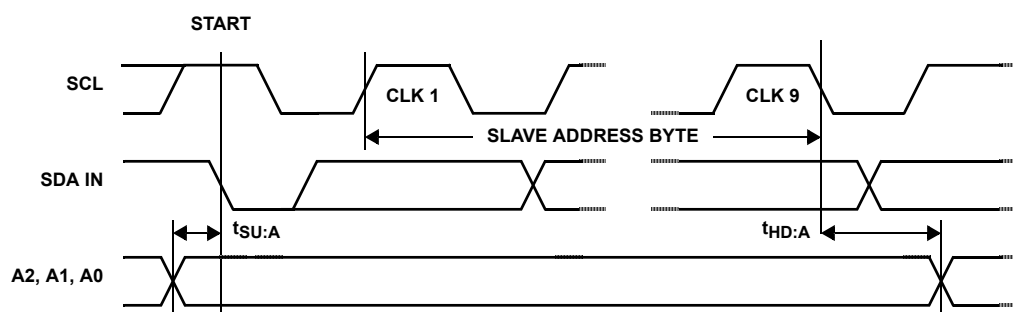
FIGURE 2. ADDRESS PIN TIMING
