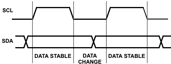
FIGURE 7. VALID DATA CHANGES ON THE SDA BUS
