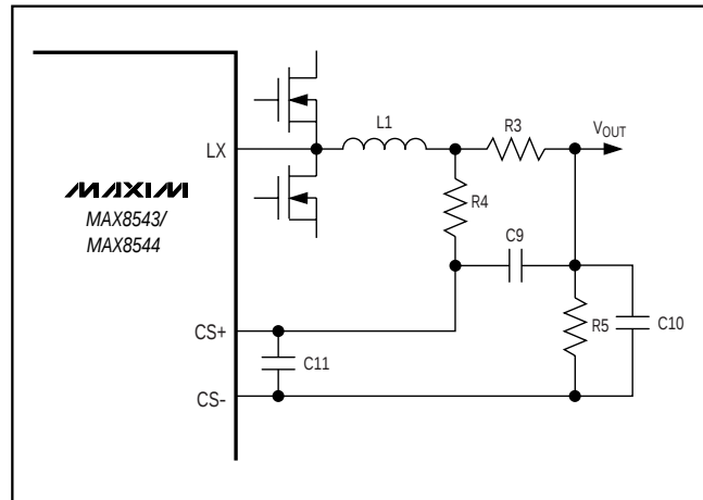
Figure 8. Using a Current-Sense Resistor
