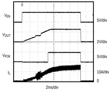
MAX8544 ENABLE WAVEFORMS
