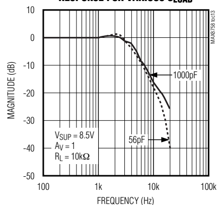
OPERATIONAL AMPLIFIER FREQUENCY RESPONSE FOR VARIOUS C_{LOAD}
