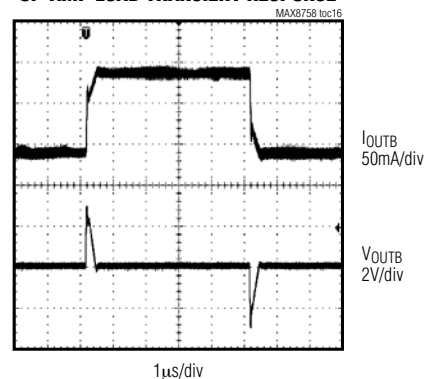
OP-AMP LOAD TRANSIENT RESPONSE
