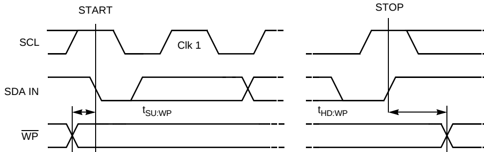
Figure 23. \overline{WP} Pin Timing
