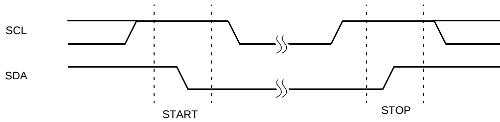
Figure 9. Valid Start and Stop Conditions
