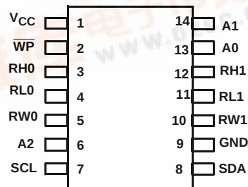
X95820 (14 LD TSSOP) TOP VIEW
