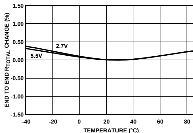
FIGURE 9. END TO END R_{TOTAL} % CHANGE vs TEMPERATURE
