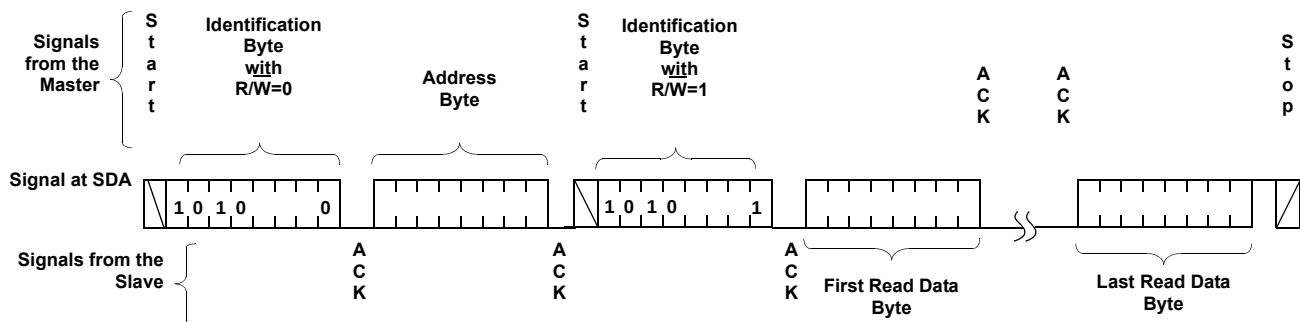
FIGURE 18. READ SEQUENCE
