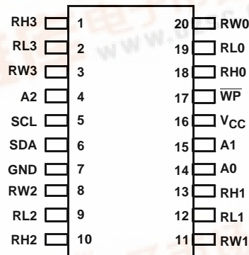
X95840 (20 LD TSSOP) TOP VIEW
