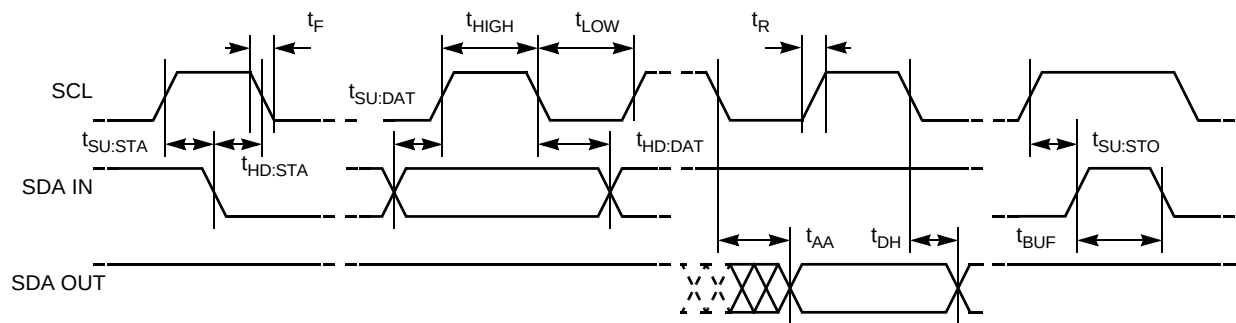
Figure 1. Bus Timing
