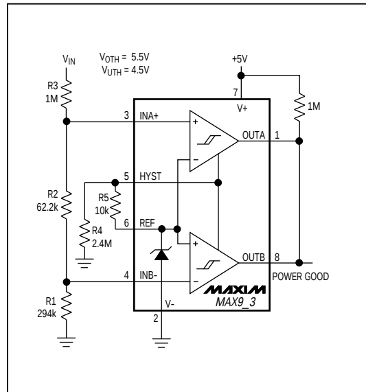
Figure 5. Window Detector
