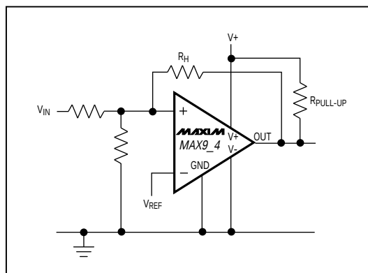
Figure 4. External Hysteresis
