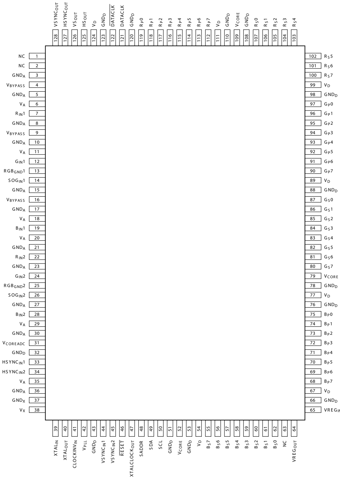
X98021 (128-PIN MQFP) TOP VIEW
