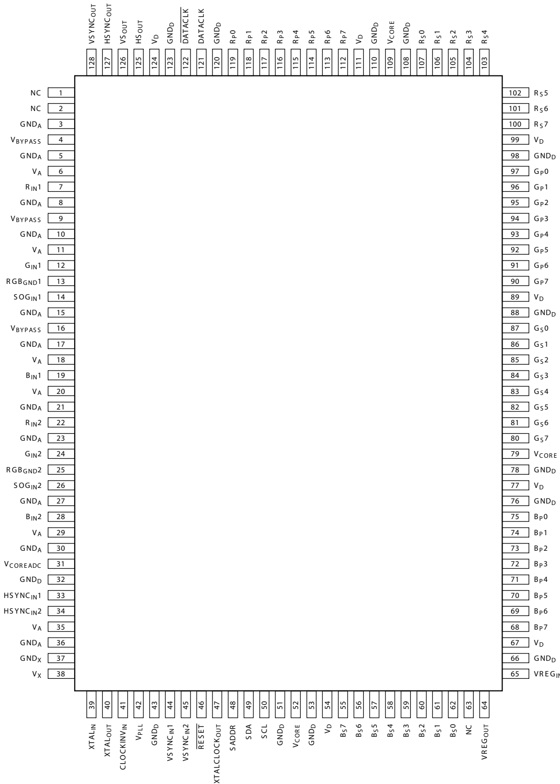
X98024 (128-PIN MQFP) TOP VIEW
