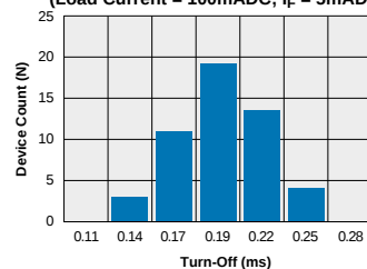
XBA170 - FormA Typical Turn-Off Time (N=50 Ambient Temperature = 25°C) (Load Current = 100mADC; I_F = 5mADC)
