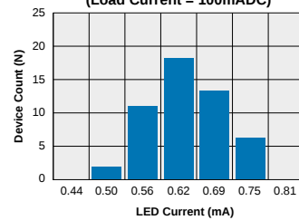
XBA170 - FormB Typical I_F for Switch Dropout (N=50 Ambient Temperature = 25°C) (Load Current = 100mADC)
