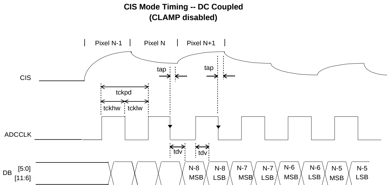
Figure 6. Timing Diagram for Figure 5
