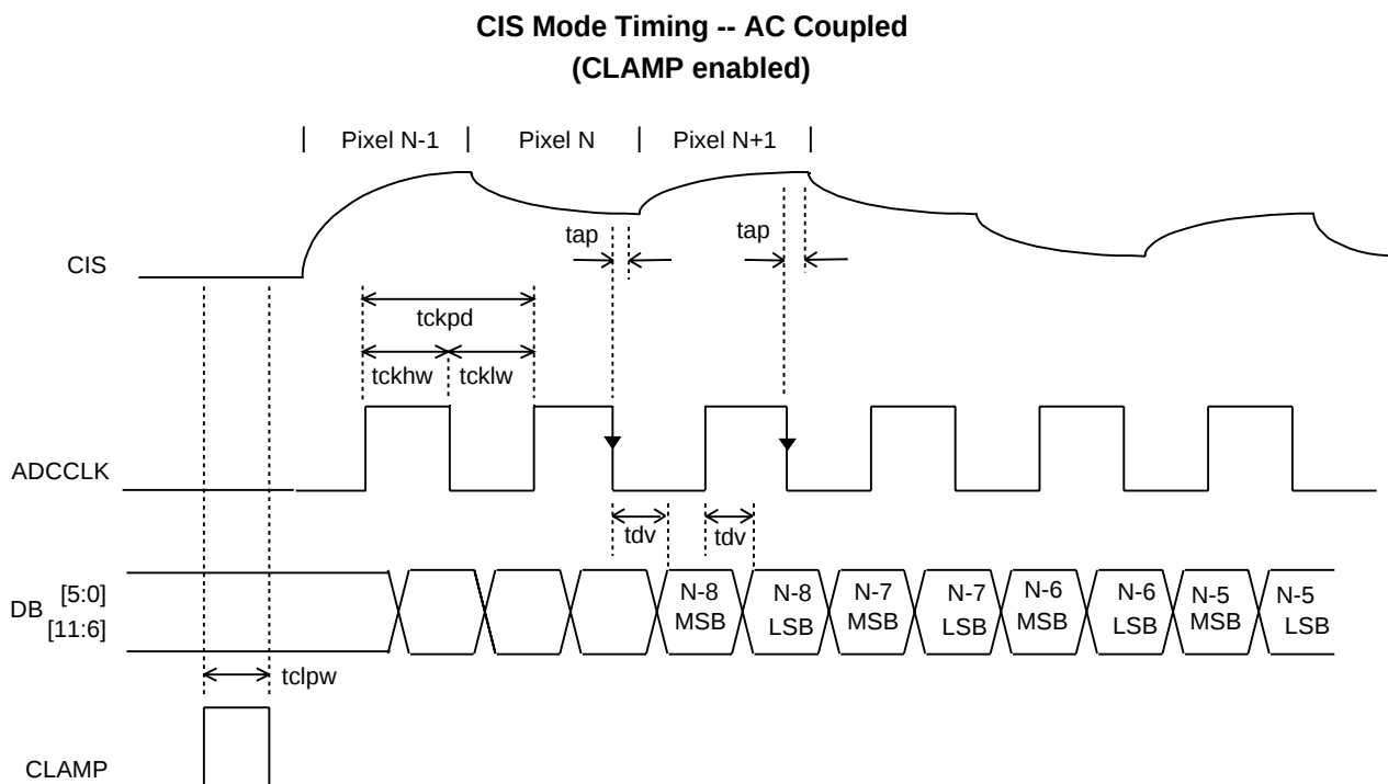
Figure 9. Timing Diagram for Figure 8
