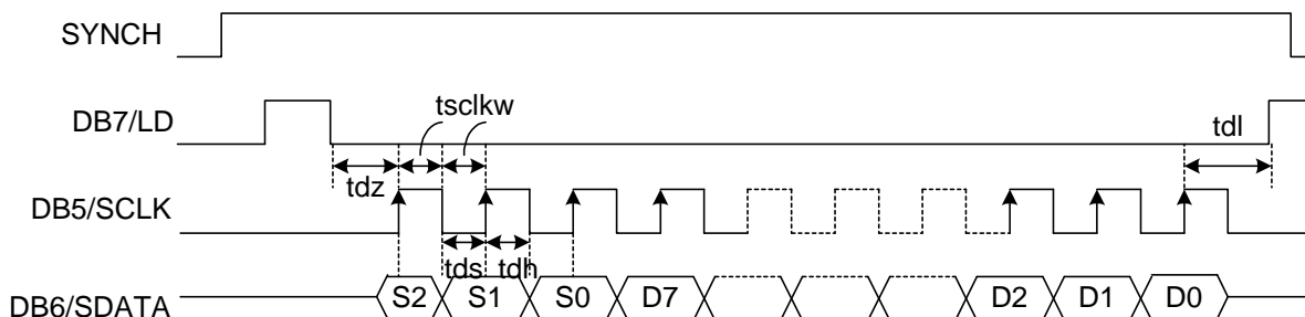
Figure 22. Write Timing
