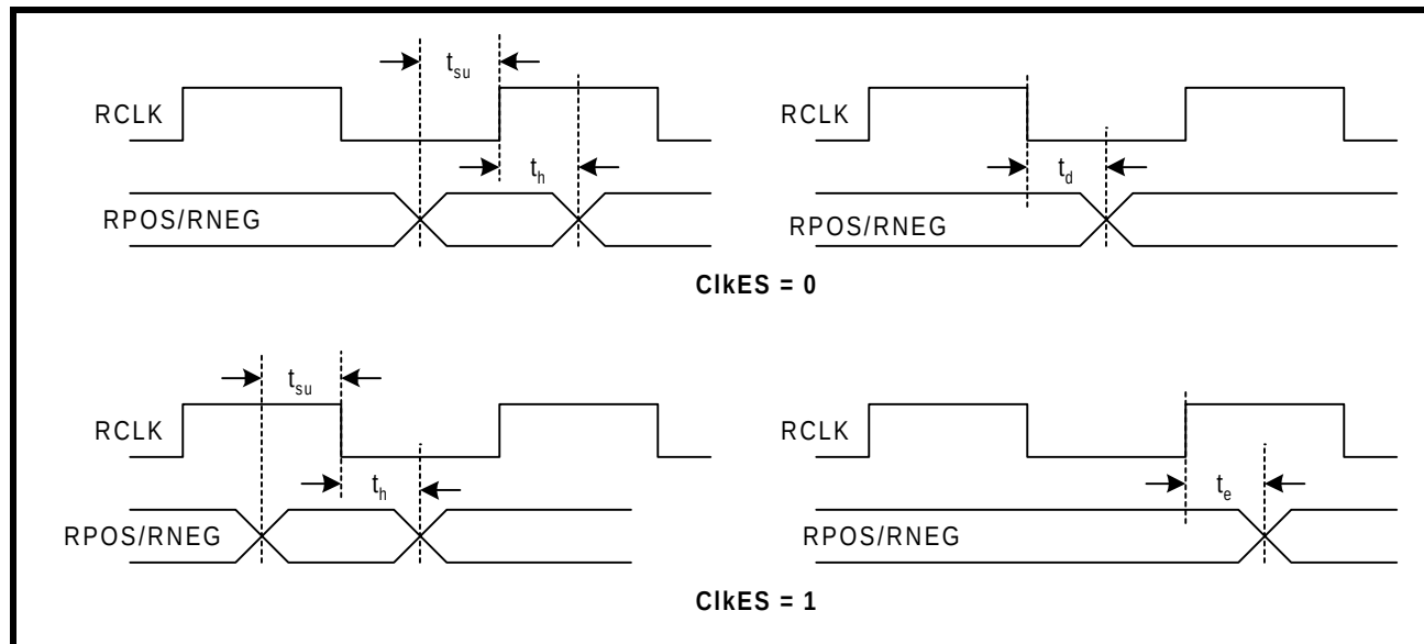
FIGURE 7. INPUT/OUTPUT TIMING
