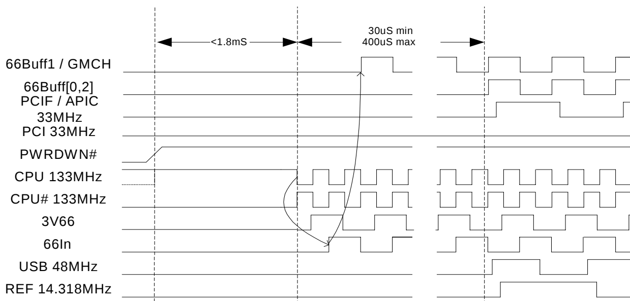
Figure 15. Power-down Deassertion Timing Waveforms – Buffered Mode
