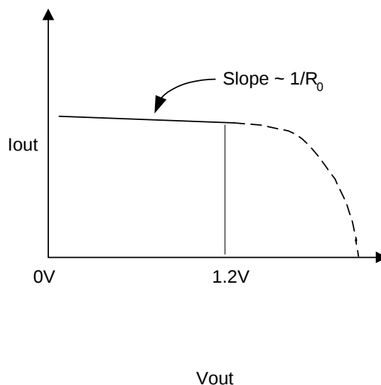
Figure 4. Buffer Characteristics
