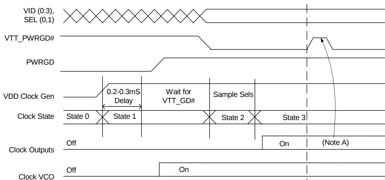
Figure 16. VTT_PWRGD# Timing
