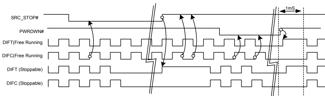
Figure 7. SRC_STOP# = Three-state, PWRDWN# = Three-state
