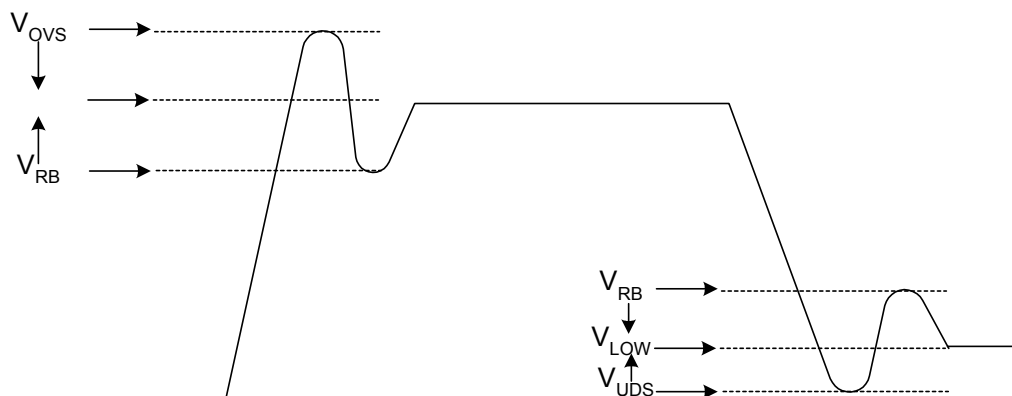
Figure 10. Single-ended Measurement Points for V_{OVS} , V_{UB} and V_{RB}
