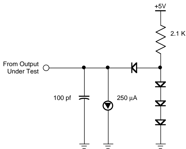
Figure 59. Standard Test Circuit
