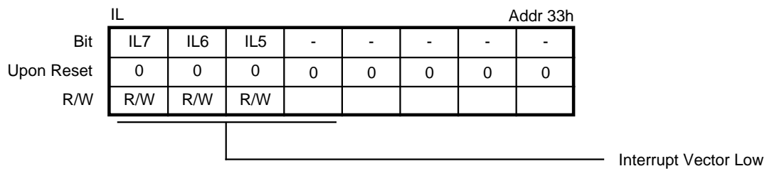
Figure 41. Interrupt Vector Low Register
