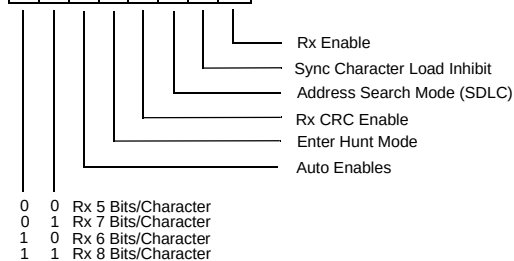
Figure 15. Write Register Bit Functions
