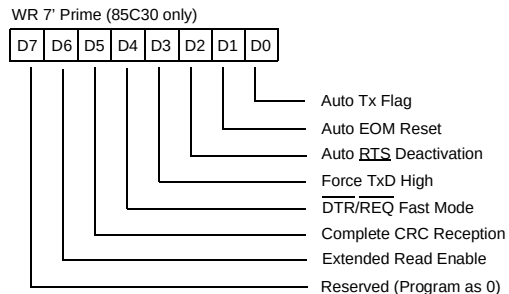
Figure 17. Write Register Bit Functions
