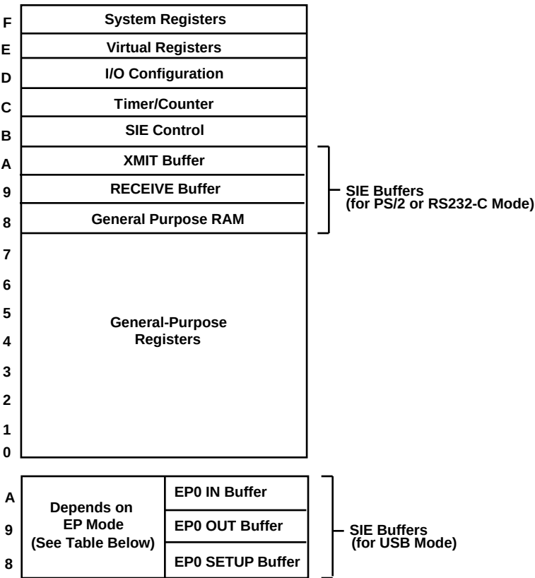
Figure 12. Register Files
