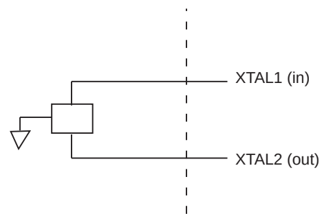
Figure 20. Oscillator Configuration
