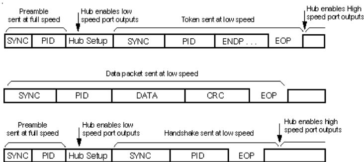
Figure 2. Data To/From Z8E520/C520
