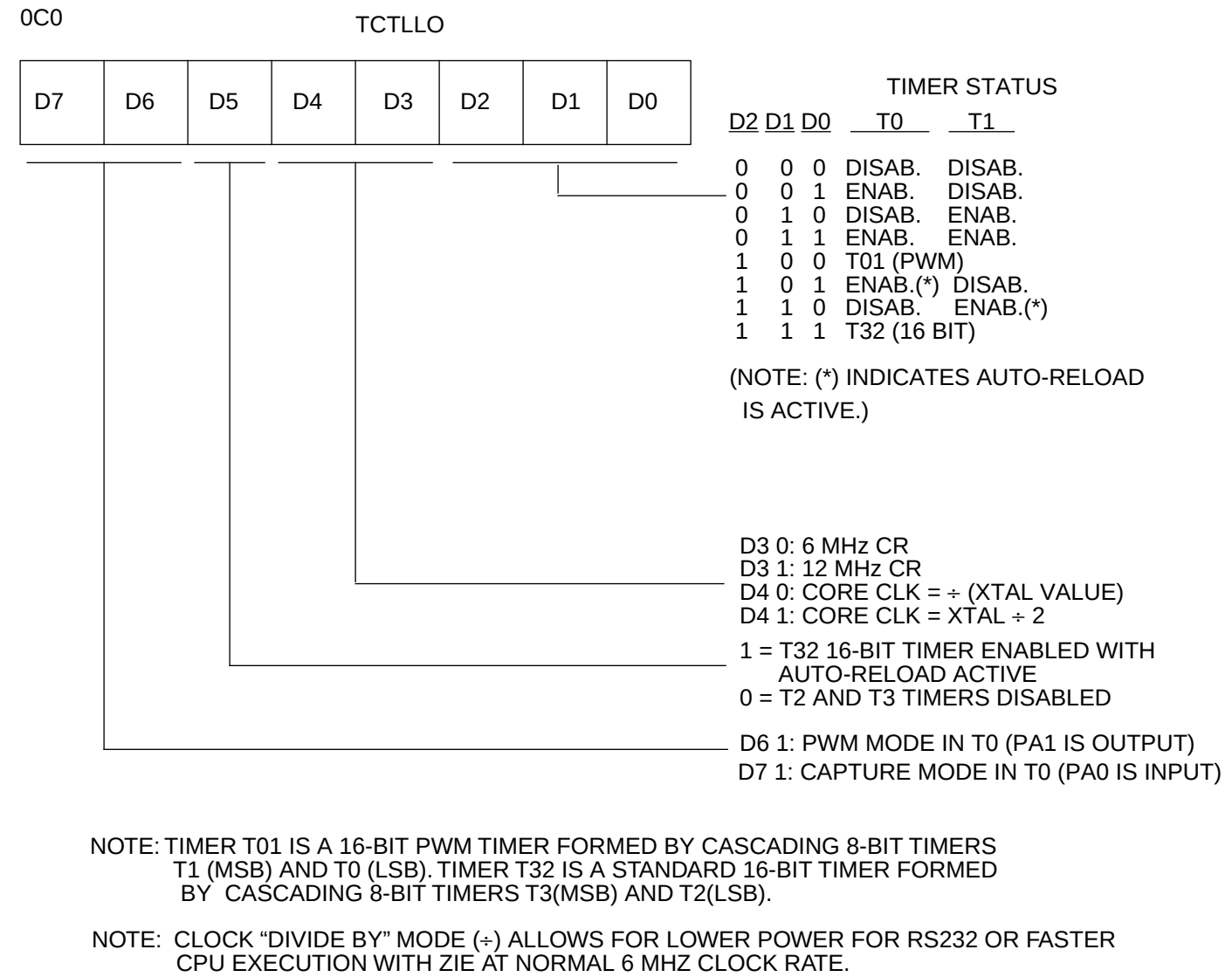
Figure 25. TCTLLO Register
