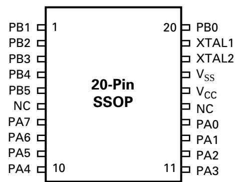
Figure 5. 20-Pin SSOP Pin Identification
