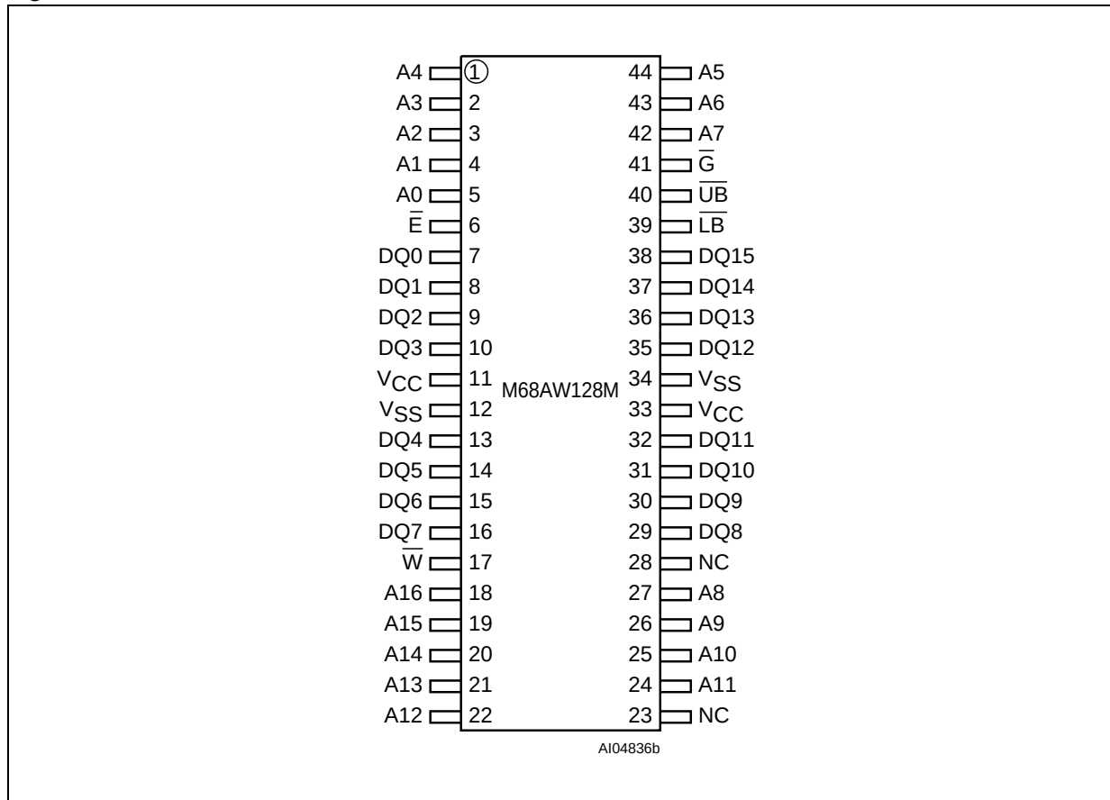
Figure 3. TSOP Connections
