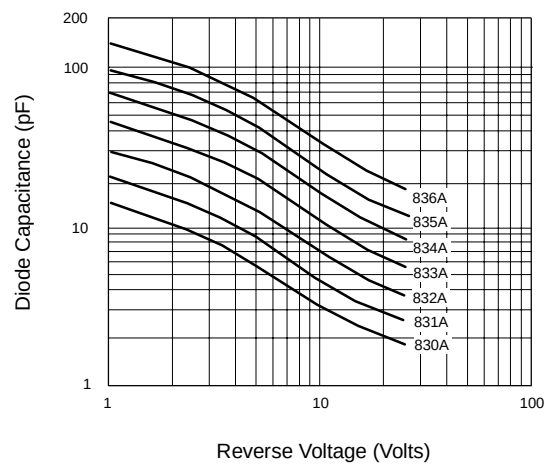
Diode Capacitance
