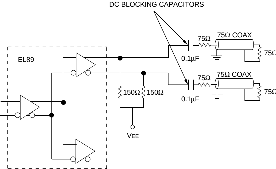
Figure 1. Termination Configuration
