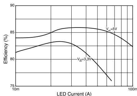
LED Current v Efficiency
